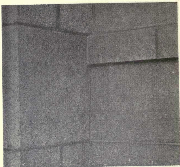
FIG. 76—NATURAL GRANITE AT LEFT OF CENTER; MANUFACTURED GRANITE AT RIGHT—DETAIL OF GORE HALL, HARVARD UNIVERSITY, WARREN AND SMITH, ARCHITECTS—EMERSON & NORRIS CO.
